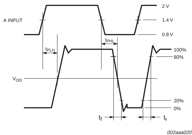
Fig 5. Propagation delay definitions.
