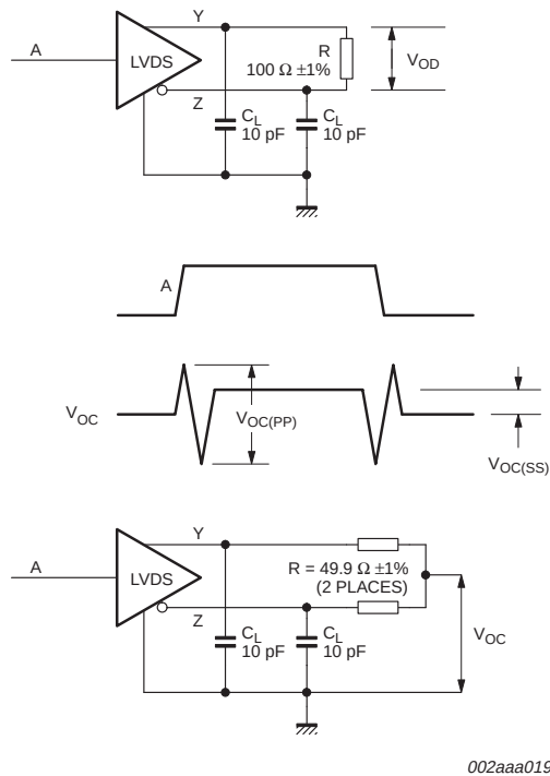
Fig 4. Test circuit and voltage definitions.
