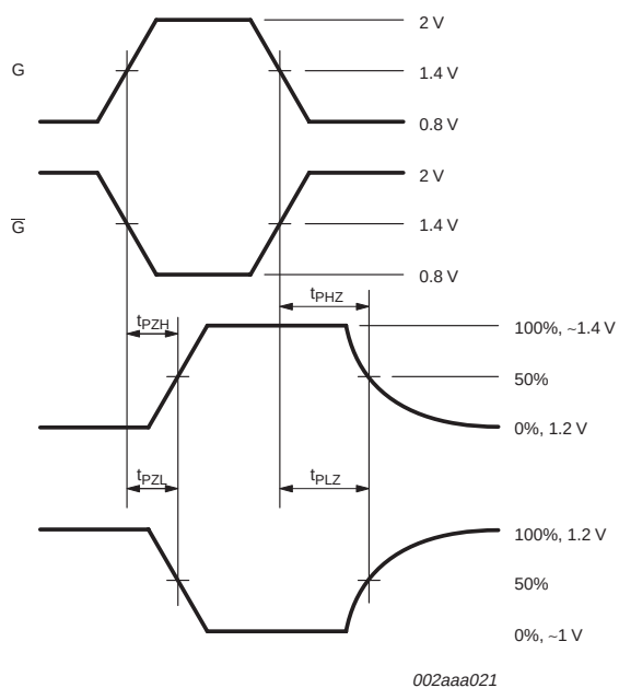
Fig 6. Enable and disable time definitions.
